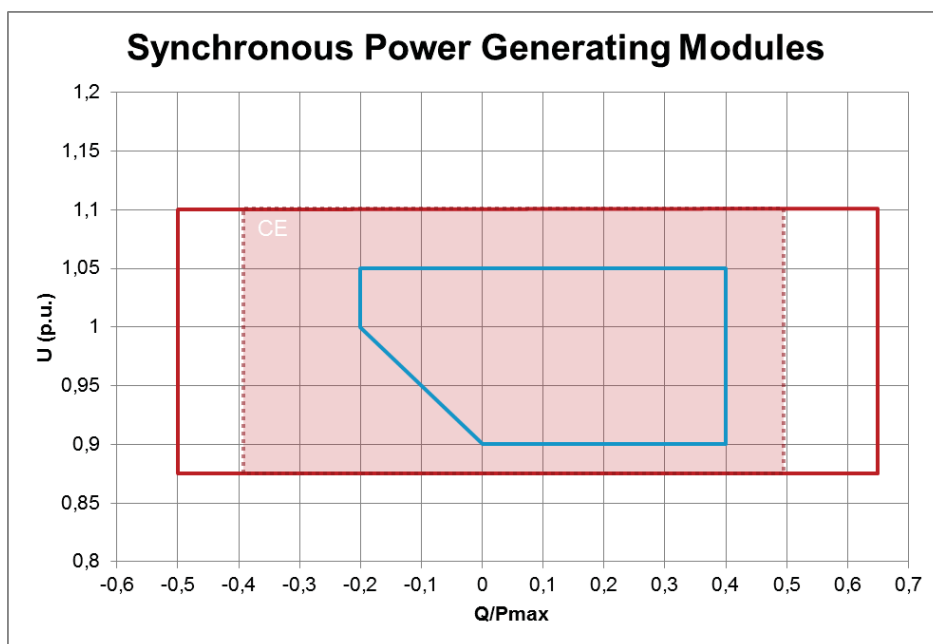
FIGURE 21 - DANISH TRANSMISSION GRID CODE ON SYNCHRONOUS GENERATORS
